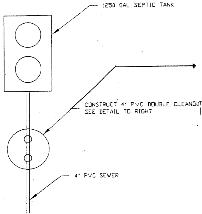
Double Cleanout Detail
