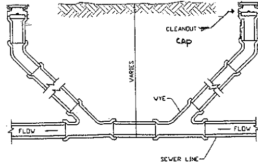
Double Cleanout Detail
