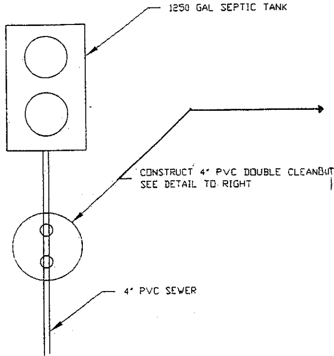
Double Cleanout Detail
